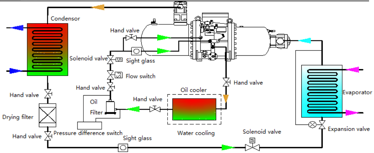
Diagram of water cooling system (single compressor)
