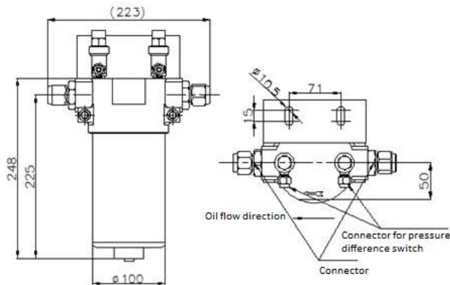
Figure-External Oil filter
